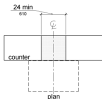
Figure 904.4 (Exception) Alteration of Sales and Service Counters
